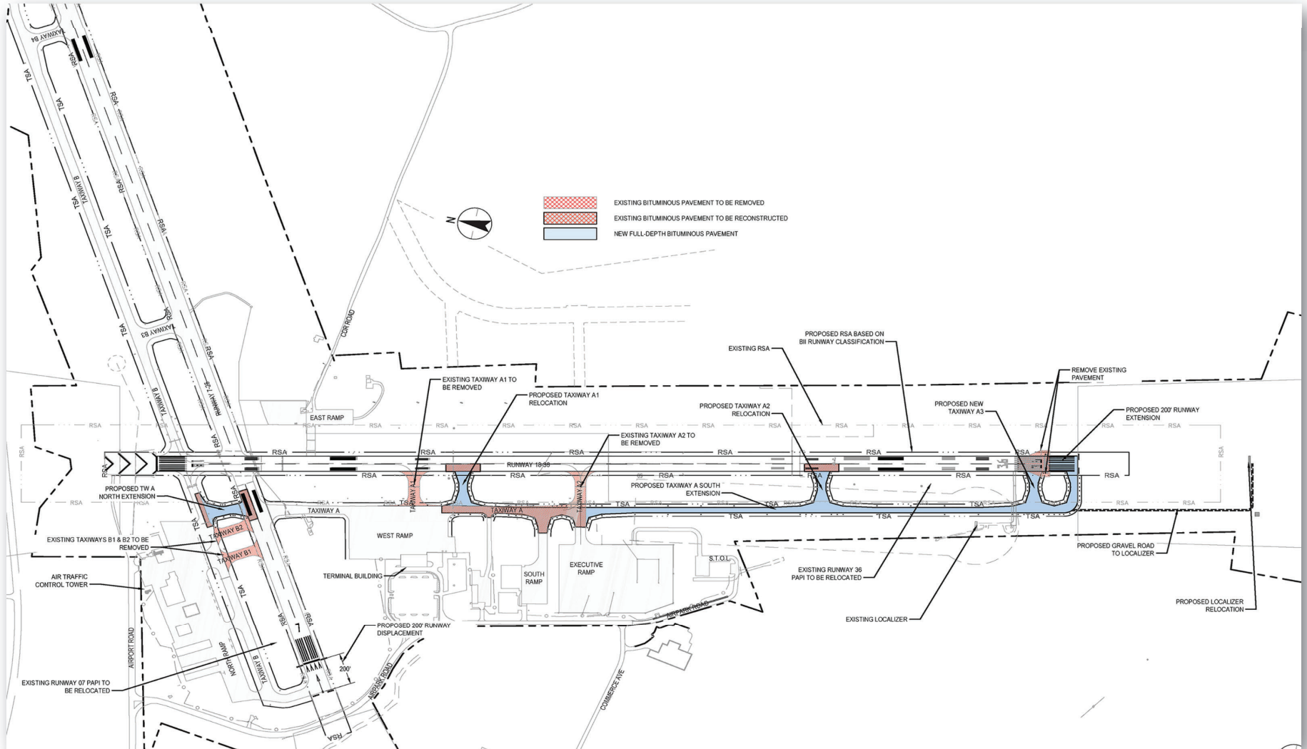
Figure 4.5. Proposed Taxiway Layout
